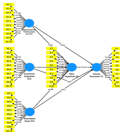
Gambar 4 Diagram Jalur SEM-PLS (Inner Model)
