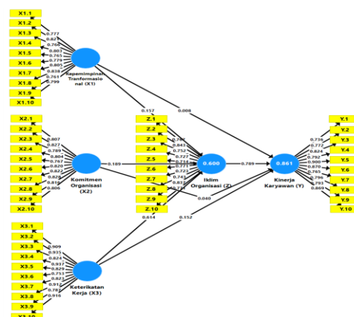
Gambar 3. Diagram Jalur SEM-PLS ( Outer Model )
